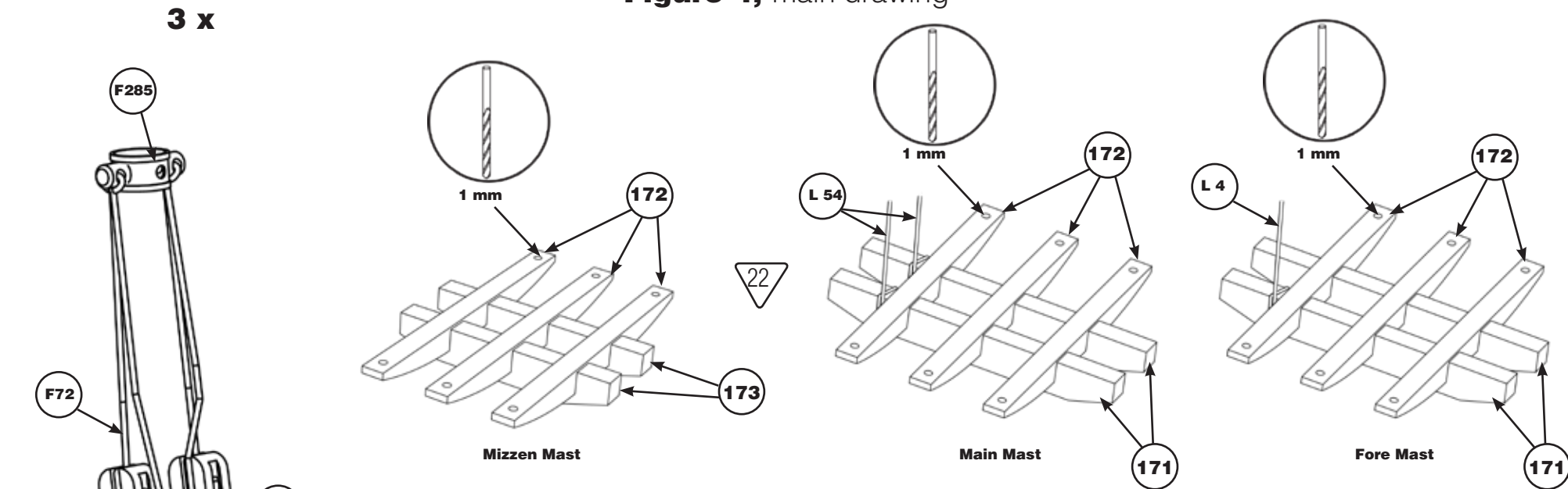
Figure 4, main drawing
