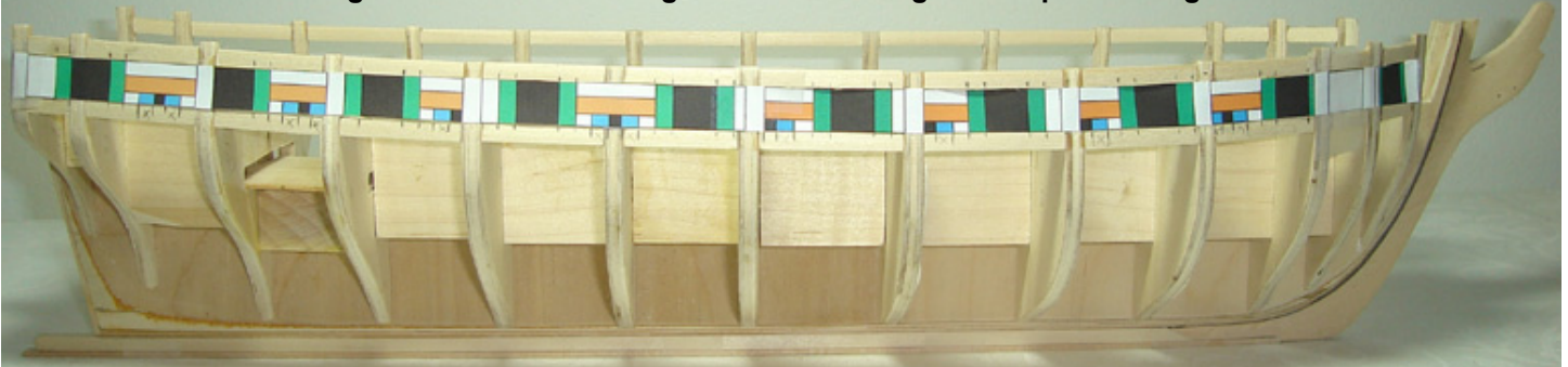
Marking the locations for the green frames using the template as a guide.
