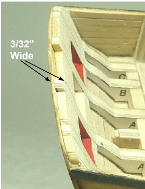
Planked inboard with 1/8" x 1/16" planks from the deck up.
