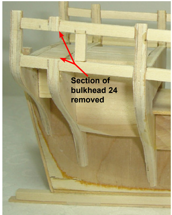
Cut bulkhead 24 out as shown to make room for the final gunport frame. Note the type of blade used.
