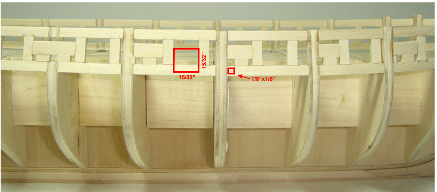
All of the red frames are glued into place. These frames define the top of each sweep port.
