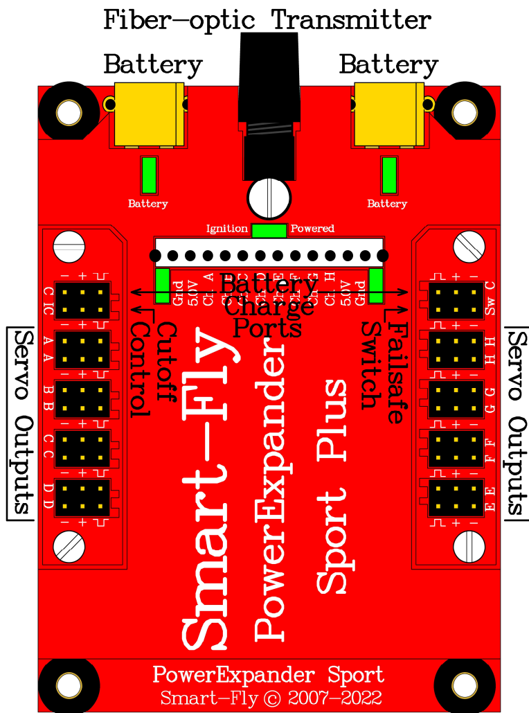
Reference Drawing
